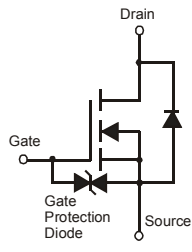
EQUIVALENT CIRCUIT
