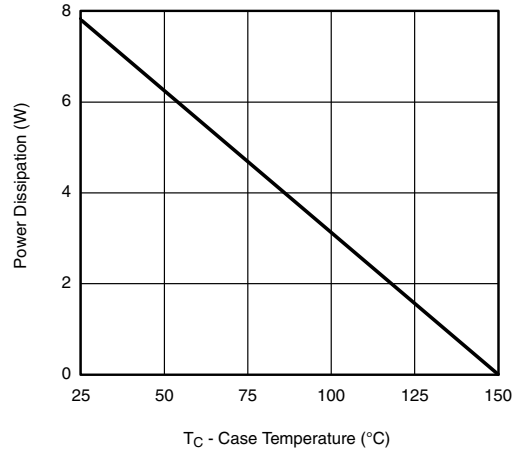
Power Derating
