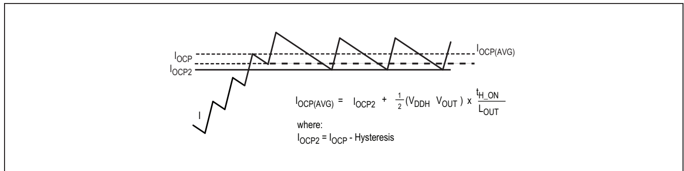
Figure 2. Inductor Current During Current Limiting
