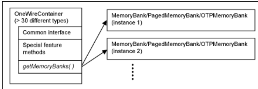
Figure 7. OWAPI ONEWIRECONTAINER features.
