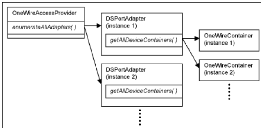
Figure 6. OWAPI object creation.
