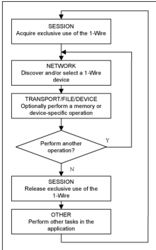
Figure 3. API usage flow.
