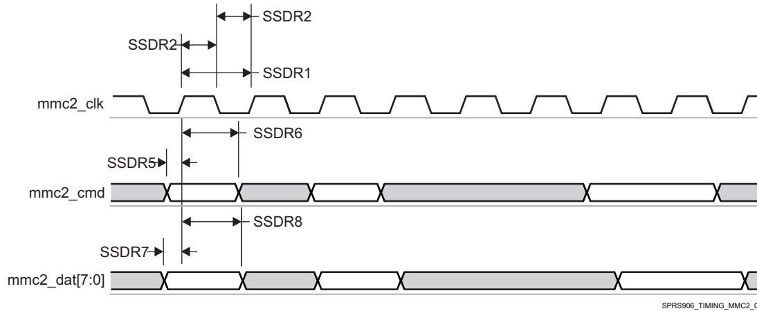
Figure 5-87. MMC/SD/SDIO in - Standard JC64 - Receiver Mode
