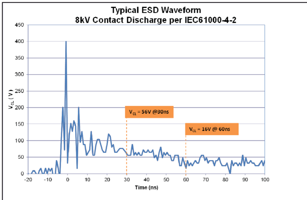
FIGURE 3. ESD WITHSTAND
