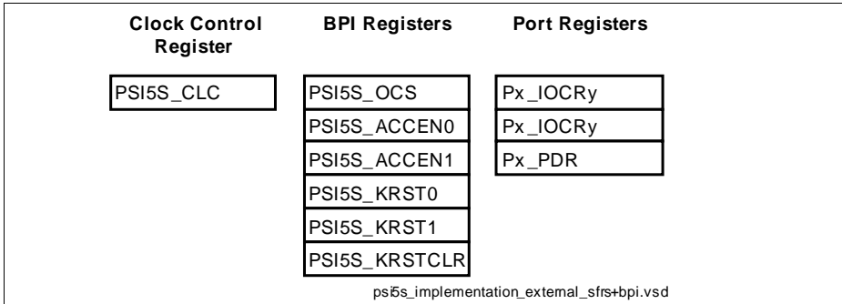
Figure 33-36 PSI5-S Implementation-specific Special Function Registers
