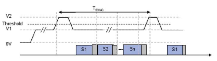
Figure 33-9 Synchronous Transmission
