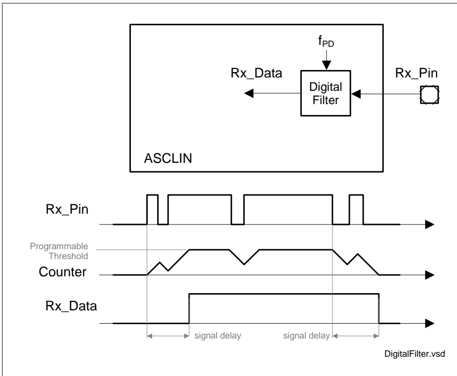
Figure 18-31 Digital Filter
