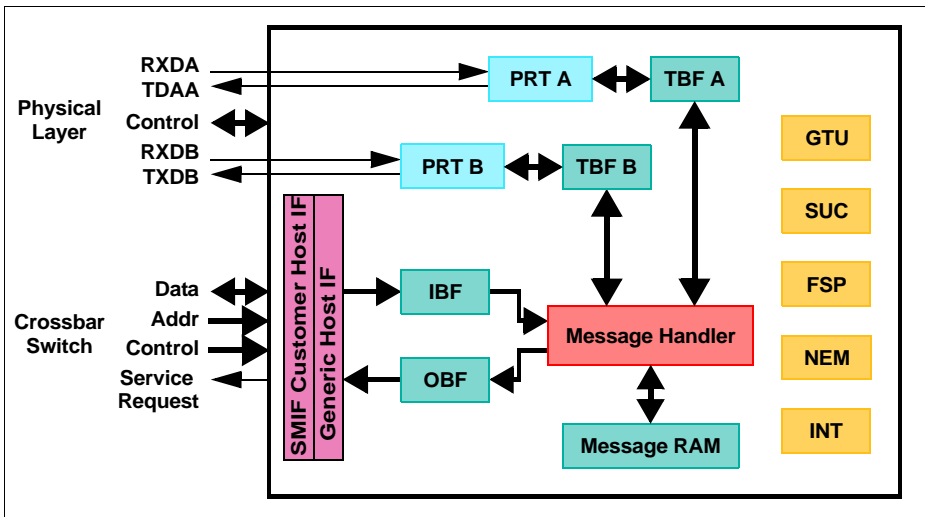
Figure 24-2 E-Ray Block Diagram
