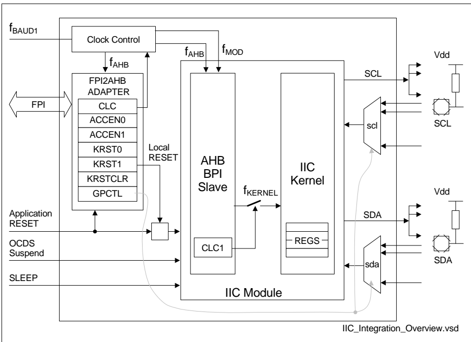
Figure 30-28 Integration Overview
