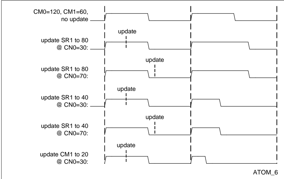
Figure 25-37 synchronous update of duty cycle
