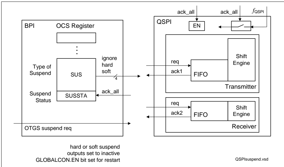
Figure 19-54 Suspend Overview
