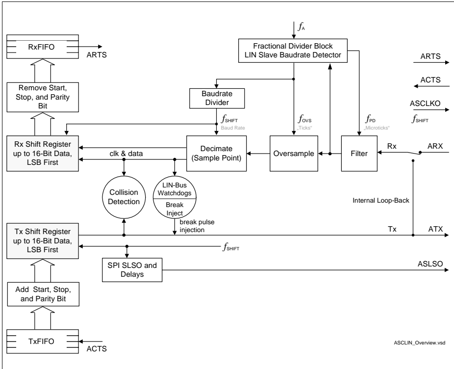
Figure 18-2 Architecture Overview
