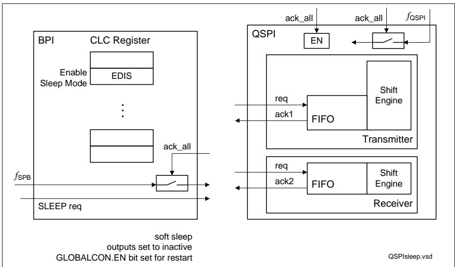
Figure 19-55 Sleep Overview
