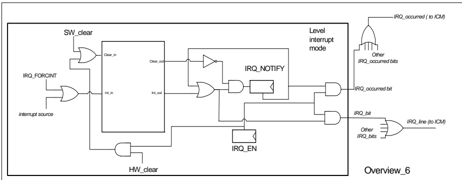
Figure 25-8 Level interrupt mode scheme
