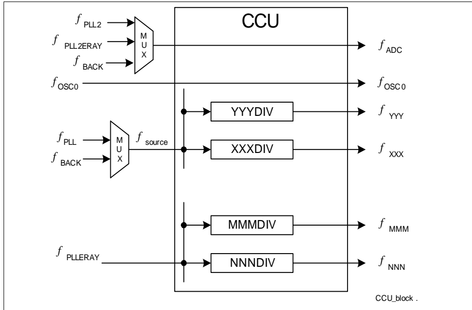
Figure 7-14 Clock Control Unit Overview
