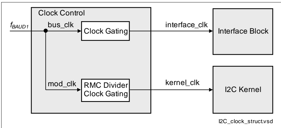
Figure 30-26 Module Clock Control
