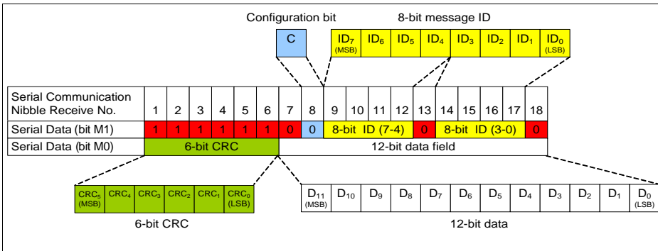
Figure 32-7 Configuration Bit = 0
