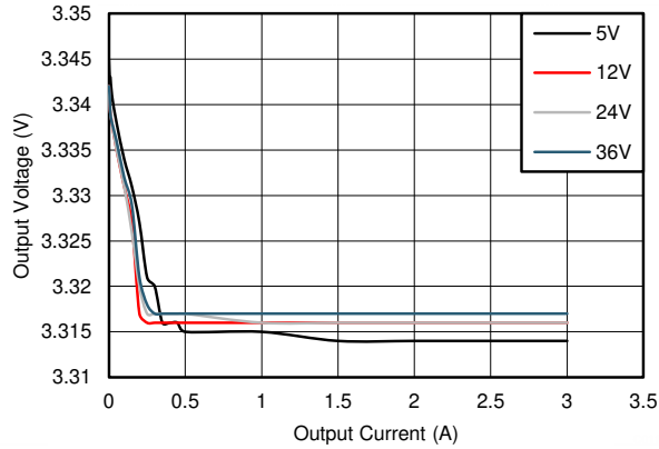
Figure 8-17. Line and Load Regulation
