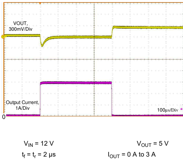
Figure 8-15. Load Transient
