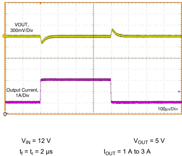
Figure 8-16. Load Transient
