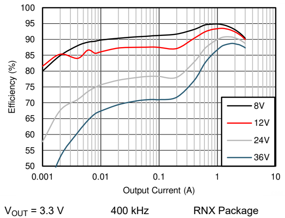
Figure 8-6. Efficiency
