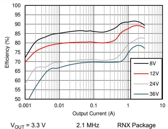
Figure 8-10. Efficiency
