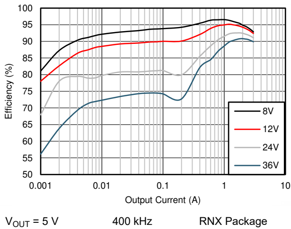
Figure 8-5. Efficiency
