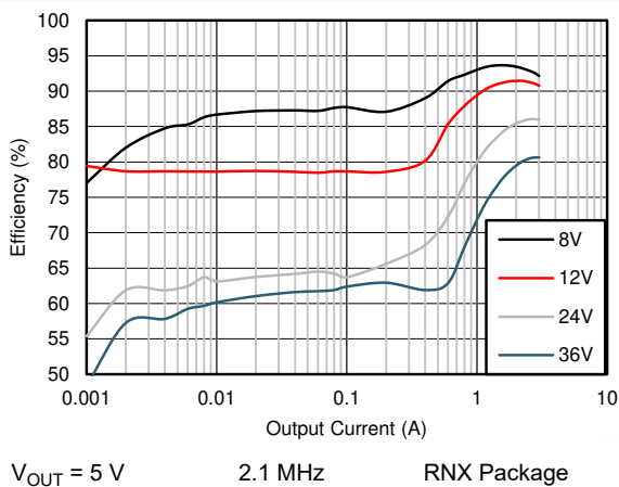
Figure 8-9. Efficiency
