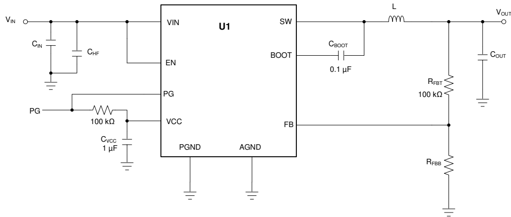
Figure 8-29. Circuit for Application Curves
