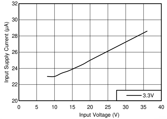
Figure 8-18. Input Supply Current
