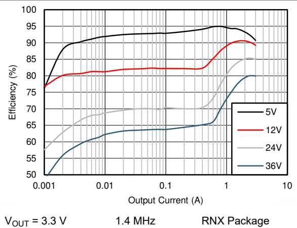
Figure 8-8. Efficiency
